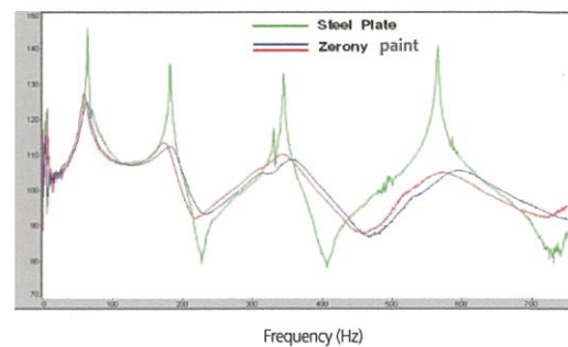
Frequency (Hz)
